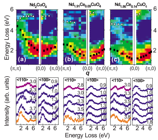
FIG. 2. (Color online) Doping evolution of charge excitations in NCCO: (a) x=0 (parent Mott state), (b) x=0.09 (doped AFM), and (c) x=0.14 (superconductor). The upper row shows intensity maps in the reduced zone by using a color scheme wherein high intensity is denoted as red (dark gray) and low intensity as blue (black). The black, gray, and white dots are guides to the eye for the dispersion of low-, medium-, and high-energy excitation branches, respectively. The lower row gives a few representative spectra corresponding to the images in the upper row. Absolute momentum values (in units of \pi/a_0 ) are shown attached to various spectra and lie in the fourth BZ along [110] and the second BZ along [100].
