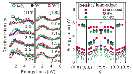
FIG. 3. (Color online) (a) Spectral curves (raw data) along [110] and [100] for the undoped system [red (dark gray) squares] are compared at various momenta to the corresponding spectra for the doped system [black circles and green (gray) diamonds]. (b) The positions of peaks [marked in Figs. 2(a)–2(c)] based on the center of gravity method (Refs. 4 and 8) of various spectral features (filled symbols) and some of the associated leading edges (open symbols) as a function of momentum and doping are plotted.
