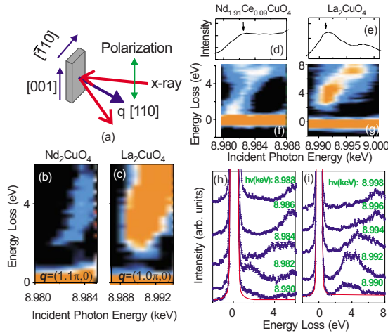
FIG. 1. (Color online) Incident energy dependence of electronic excitations. (a) Vertical scattering geometry employed with an x-ray field along [001]. [(b) and (c)] X-ray energy dependence of inelastic excitations for \text{Nd}_2\text{CuO}_4 and \text{La}_2\text{CuO}_4 . The Q values are chosen to minimize the large quasielastic background. [(d)–(g)] Excitations near the Mott gap are seen to be enhanced near the first absorption peak, not only in the undoped insulator but also in the doped system. A few energy-loss curves corresponding to the data images in (f) and (g) are shown in (h) and (i). The red (dark gray) curves show the fits to the quasielastic data.
